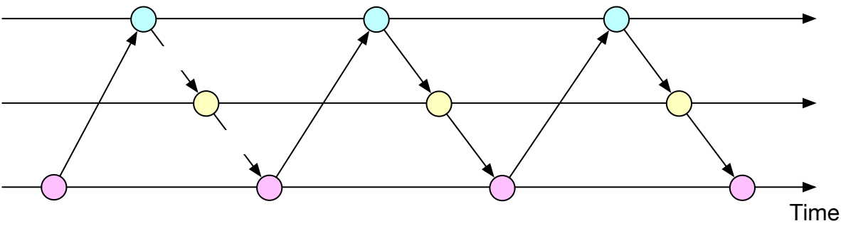
Figure 15 Dynamic view of event sourcing
