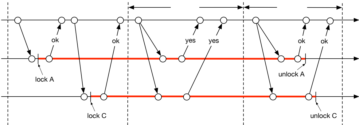
Figure 5 Two-phase commit (source [5])
