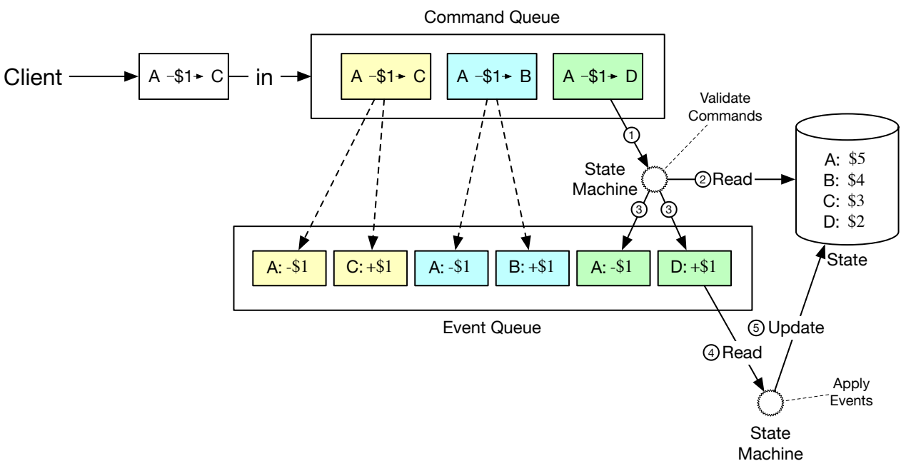
Figure 17 How state machine works
